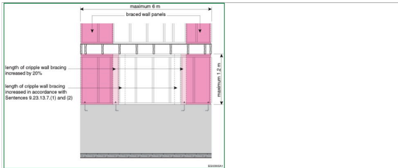
Figure A-9.23.13.8.(2) Foundation Cripple Walls Where S_{\text{max}} \leq 0.60
