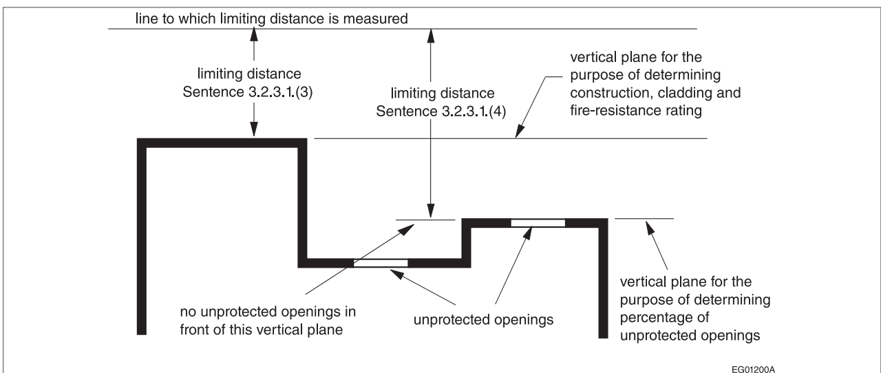
Figure A-3.2.3.1.(4) Spatial separation design
