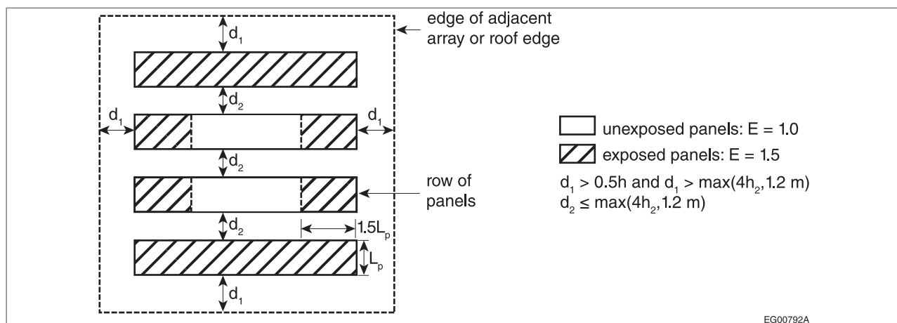
Figure A-4.1.7.13. Plan view of a roof-mounted solar array with exposed and unexposed panels
