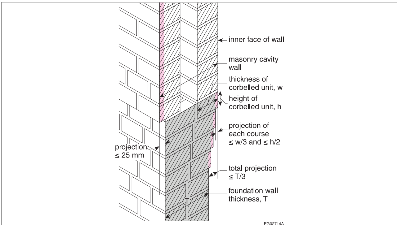
Figure A-9.20.12.2.(2) Maximum corbel dimensions
