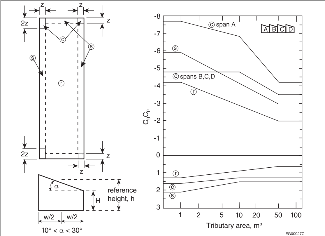
Figure 4.1.7.6.-H External peak values of C_g C_p on sawtooth roofs with a slope greater than 10^\circ for the design of structural components and cladding Forming Part of Sentence 4.1.7.6.(9)
