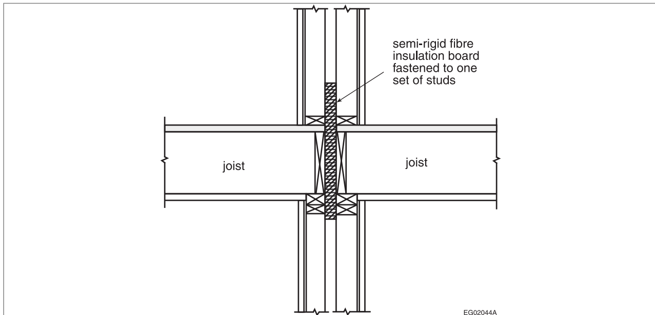
Figure A-3.1.11.7.(8) Fire block
