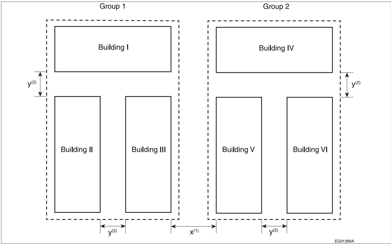
Figure A-3.9.2.2. Spatial separation between self-service storage buildings
