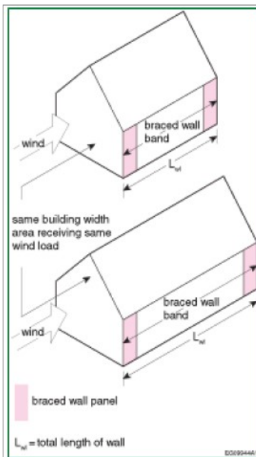
Figure A-9.23.13.7.(3) -A Wind Force on Different Length Buildings
