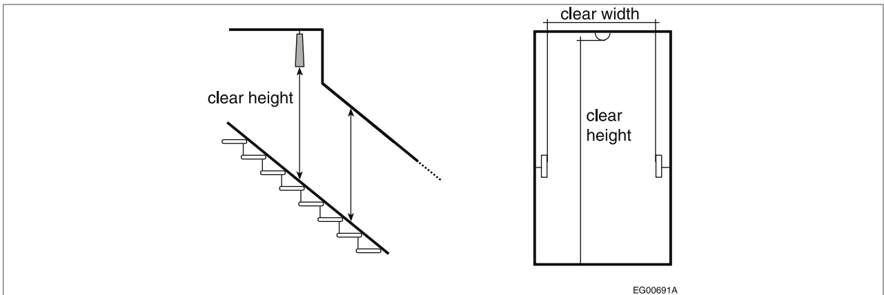
Figure A-3.4.3.4. Measuring clear height
