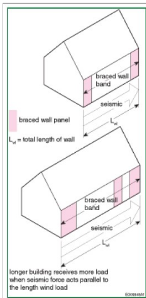
Figure A-9.23.13.7(4)-A Seismic Force on Different Length Buildings
