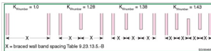
Figure A-9.23.13.7.(3) -C Adjustment for number of braced wall bands resisting wind load
