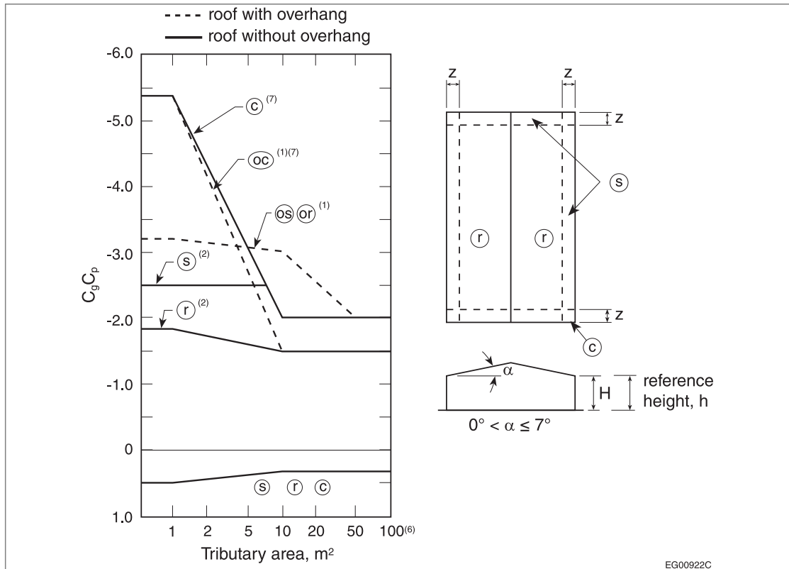
Figure 4.1.7.6.-C External peak values of C_g C_p on roofs with a slope of 7^\circ or less for the design of structural components and cladding Forming Part of Sentences 4.1.7.6.(4), (7), (8) and (9)
