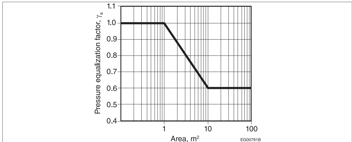
Figure 4.1.7.13.-A Pressure equalization factor, \gamma_a , for solar panels or arrays mounted on roofs of buildings of any height
