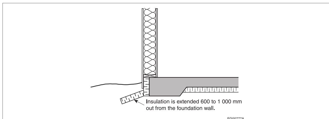
Figure A-9.36.2.8.(9) Skirt insulation
