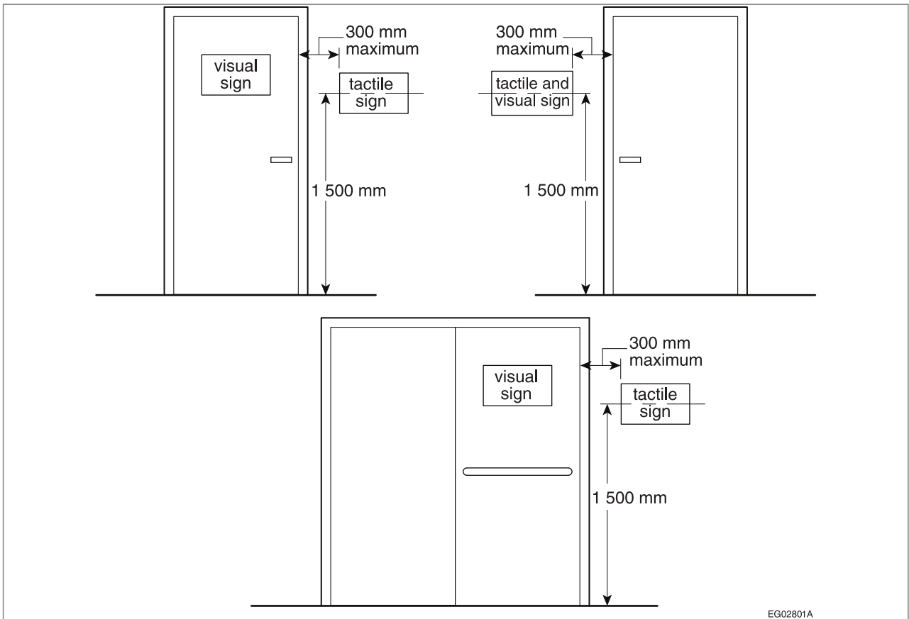
Figure A-3.8.3.9.(1) and (2)
