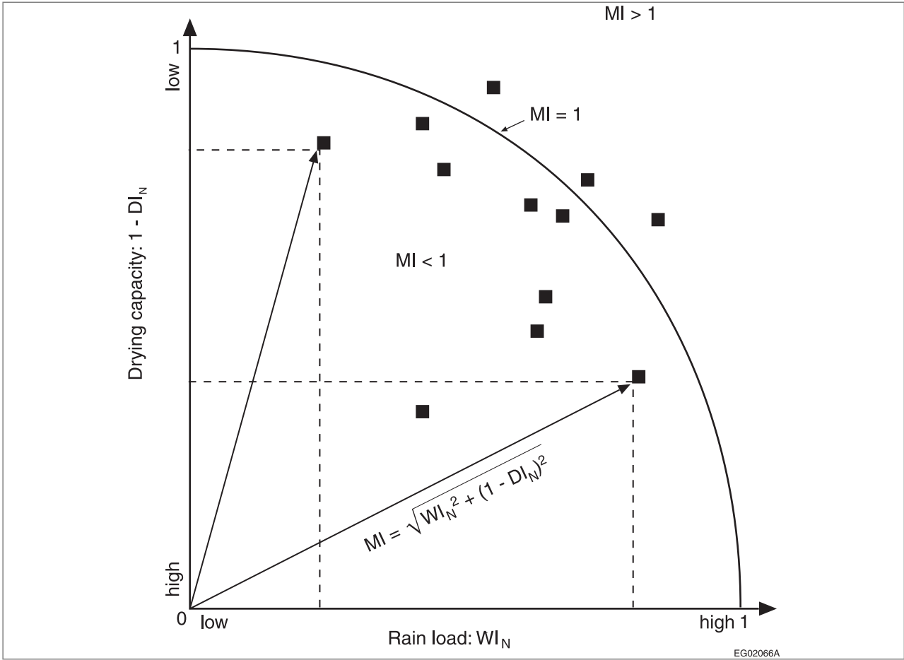
Figure C-1 Derivation of moisture index (MI) based on normalized values for wetting index (WI) and drying index (DI)
