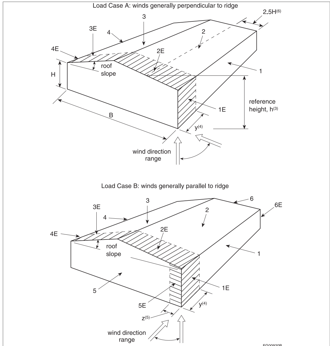
Figure 4.1.7.6.-A Primary structural actions arising from wind load acting simultaneously on all surfaces of low buildings ( H \leq 20 m)
