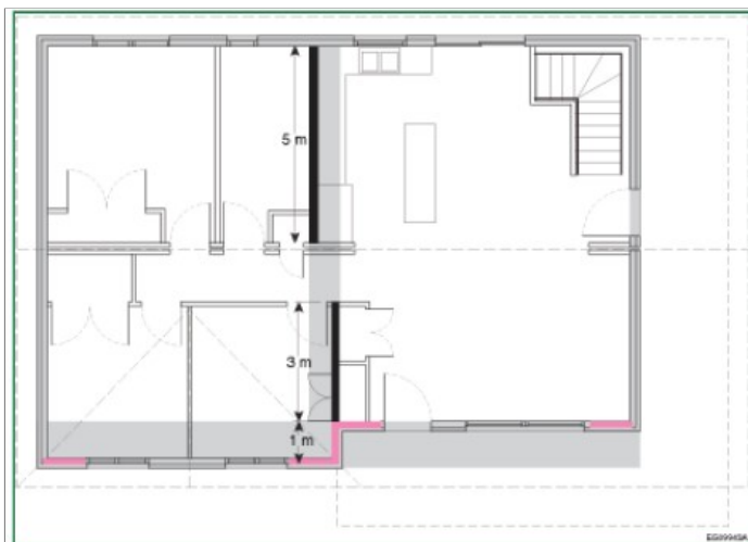
Figure A-9.23.13.6.(5) -B Mixed sheathing types in all braced wall panels using direct length substitution approach
